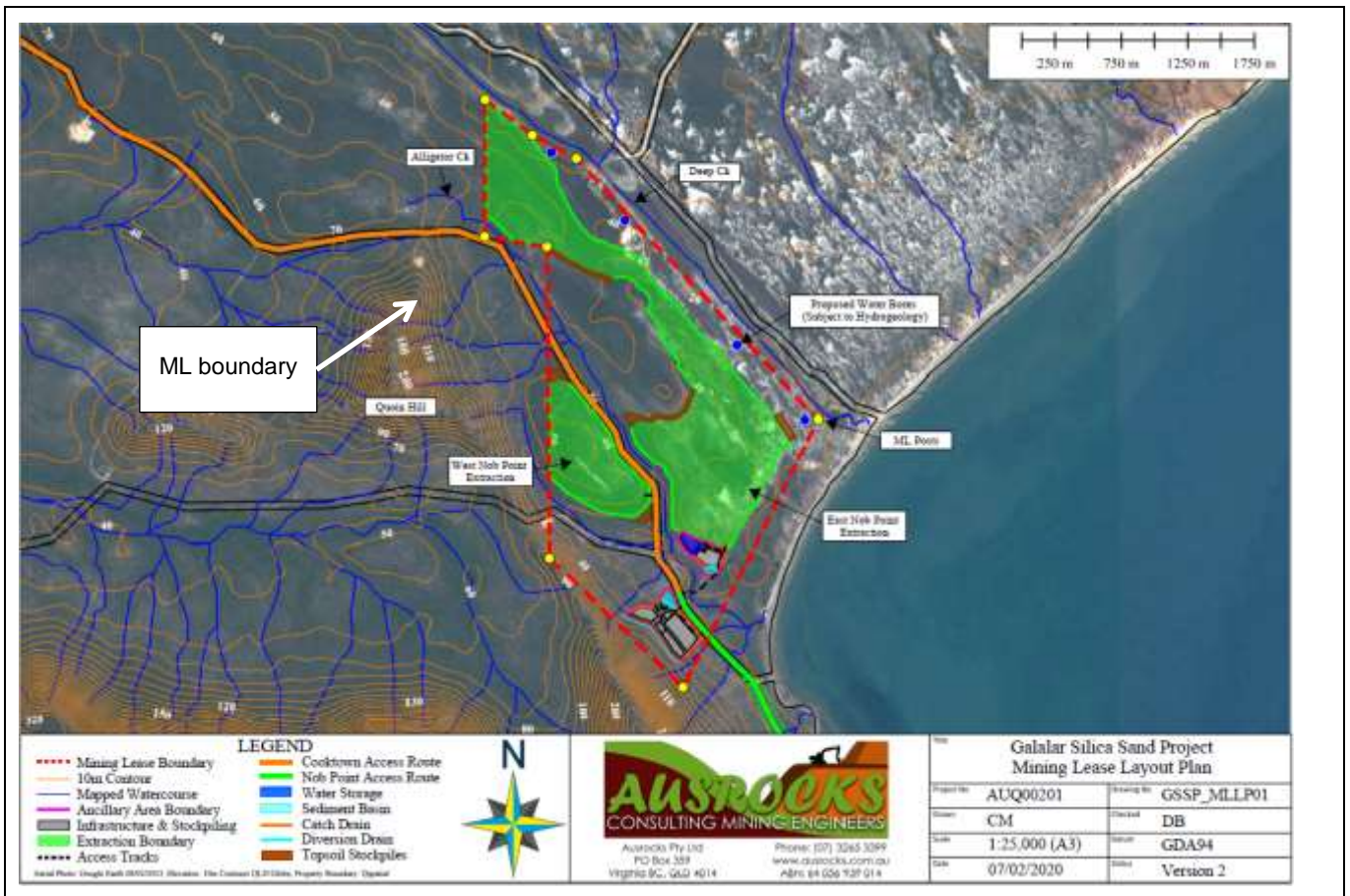
Figure 1-1 Mine and ML details.
