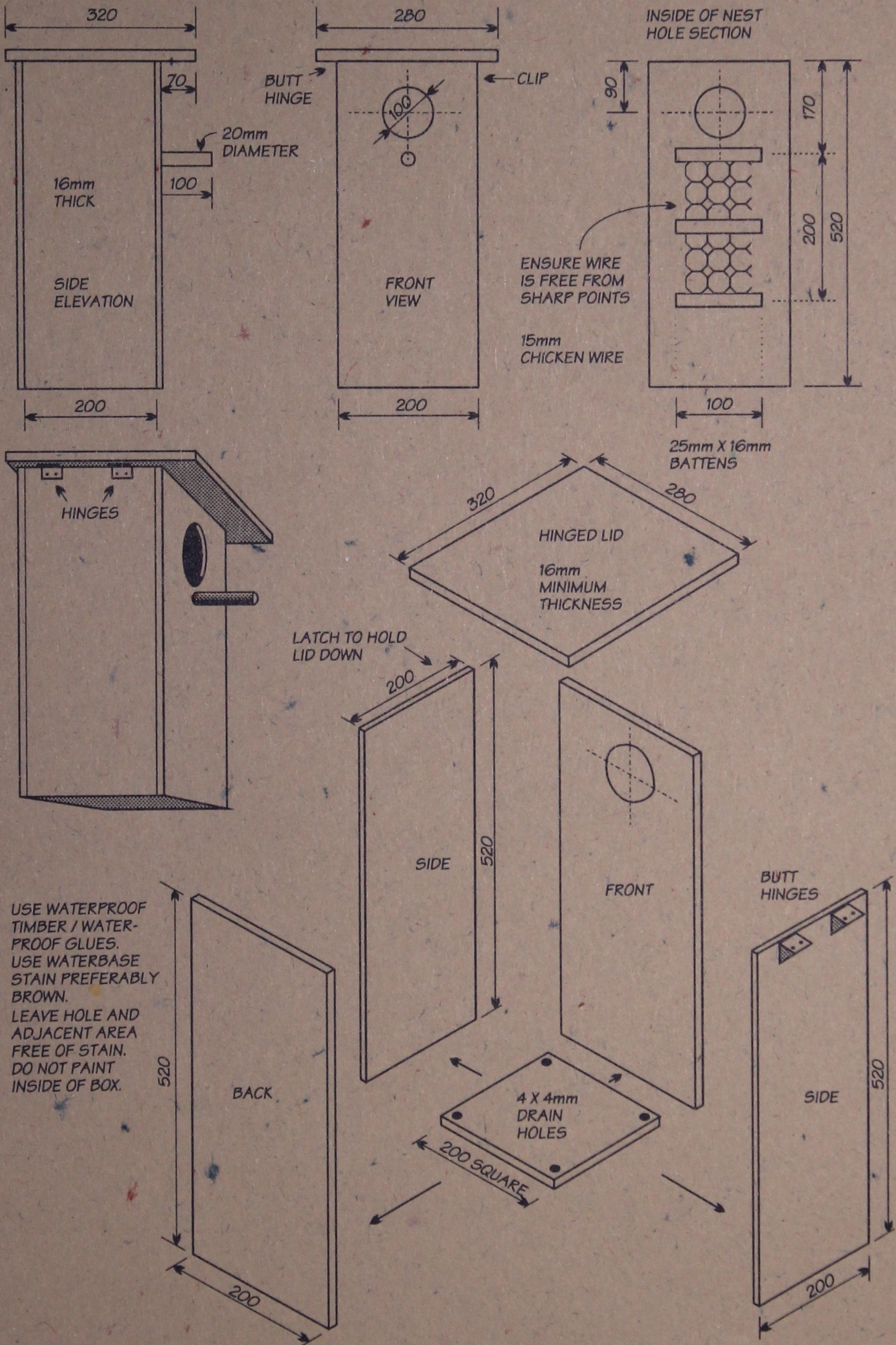
Figure D : Nesting box plans suitable for a possum
